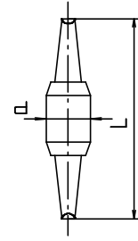
WD4 with bowl tip
